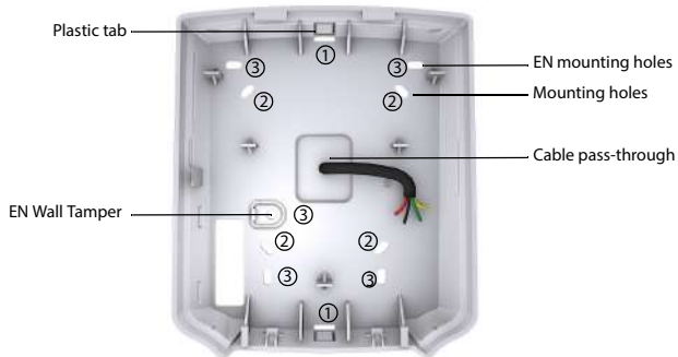
Figure 3: K32LCD+ Backplate
