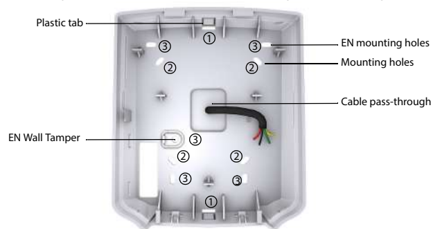
Figure 3: K32LCD+ Backplate
